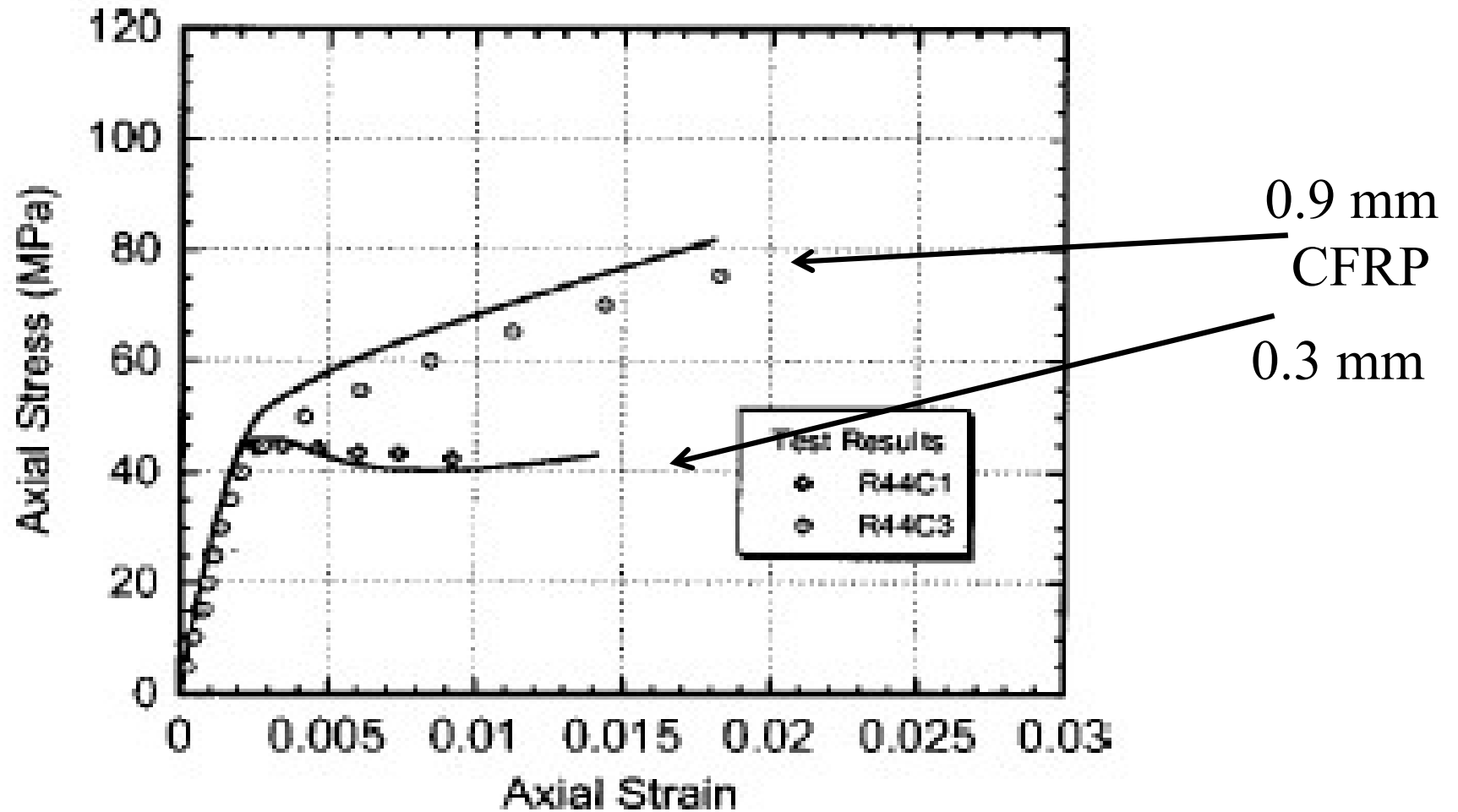
Comparison of analytical model with test results of Demers and Neal (1994)
