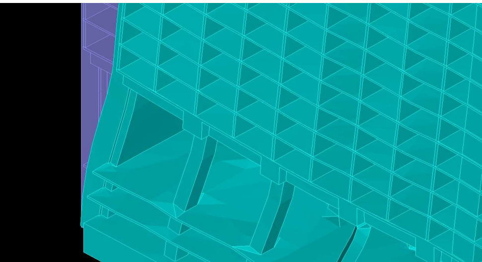
Externally Bonded FRP: Confinement
